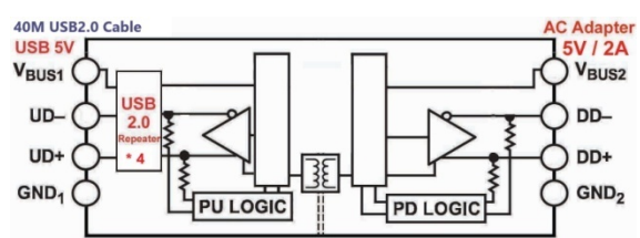
CRP-401-I Self Power-5V-2A
