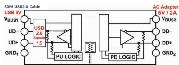
50M Type-C Isolator Active cable
