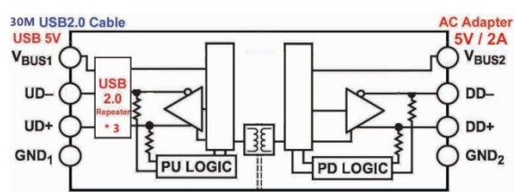
CRP-301-I Self Power-5V-2A
