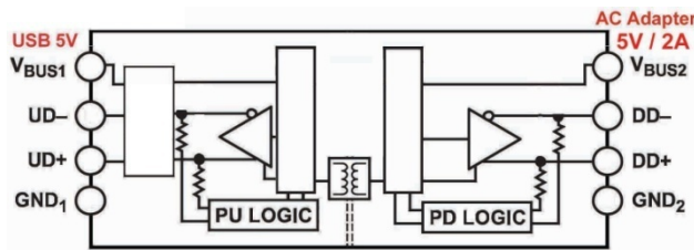
CRP-011-I Self Power-5V-2A
