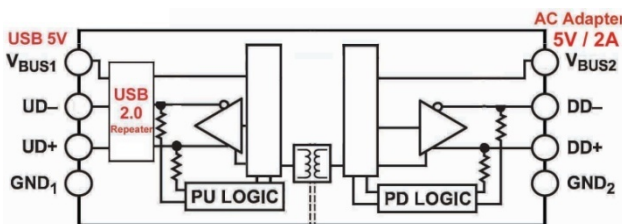
CRP-401-I Self Power-5V-2A
