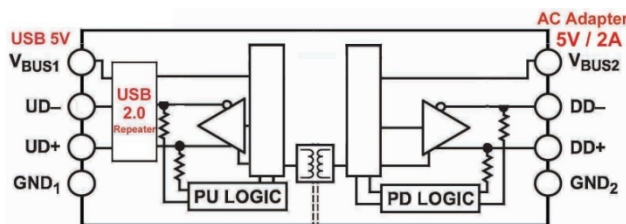
CRP-301-I Self Power-5V-2A
