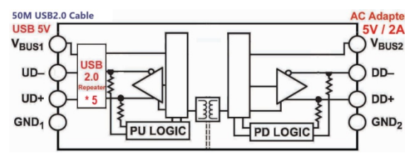
50M USB2.0 Isolator Active cable
